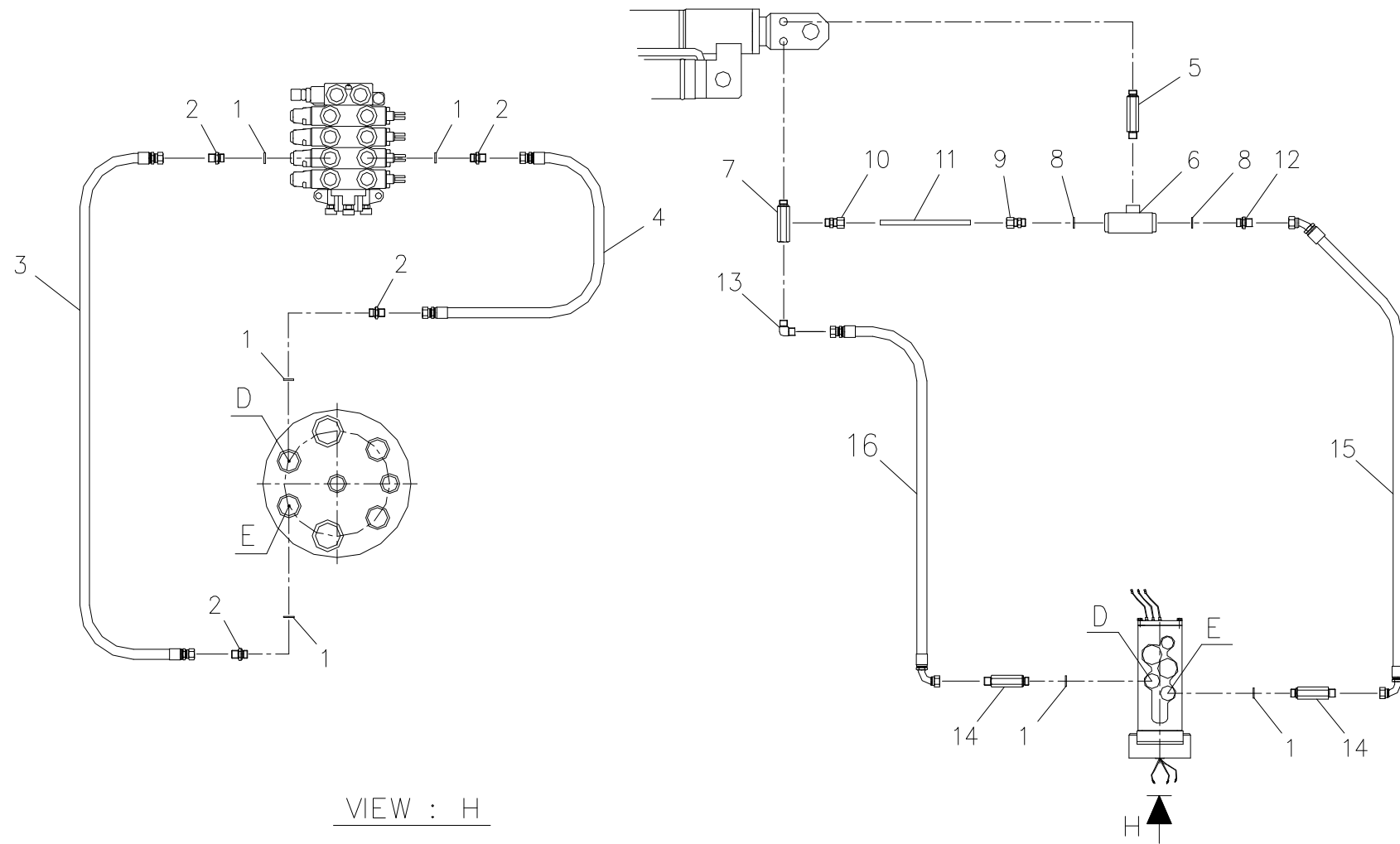
텔레스코픽 배관 (표준형) Fig. 5-4 SCS746L TELESCOPIC PIPING (STD) TEL' CYL
