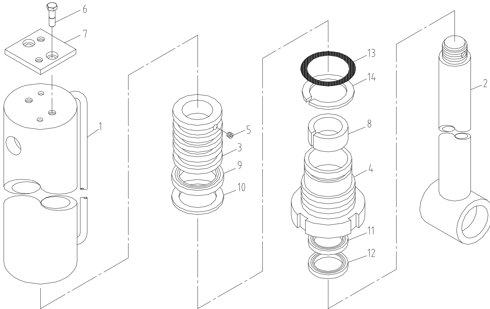
Fig. 4-1 SCS746L JACK CYL' ASS'Y
